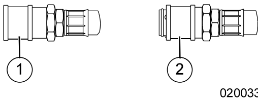
Figure 2-19. Slidable Sleeve
