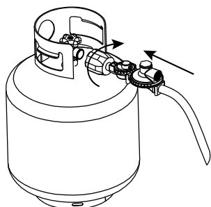
Figure 2-14. Connect Hose Assembly to LP Tank
