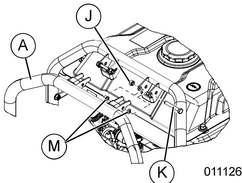
Figure 2-10. Handle Assembly
