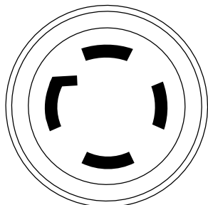
Figure 2-6. 120/240 VAC, 30 Amp Receptacle NEMA L14-30R
