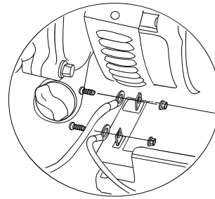
Figure 4-5. Battery Connection
