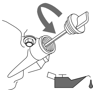
Figure 4-1. Engine Oil Fill
