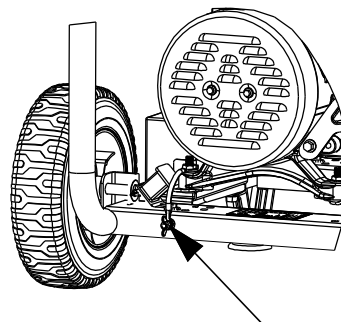
Figure 3-1. Grounding the Generator
