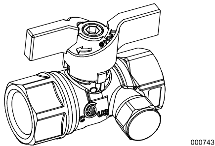
Figure 2-18. Fuel Shutoff Valve with Manometer Port
