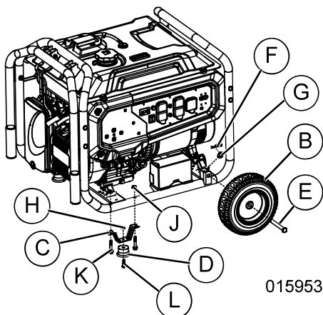
Figure 2-9. Wheel & Foot Assembly
