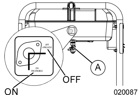
Figure 3-2. Fuel Shut-off Valve
