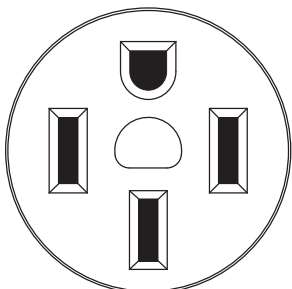
Figure 2-7. 120/240 VAC, 50 Amp Receptacle NEMA 14-50
