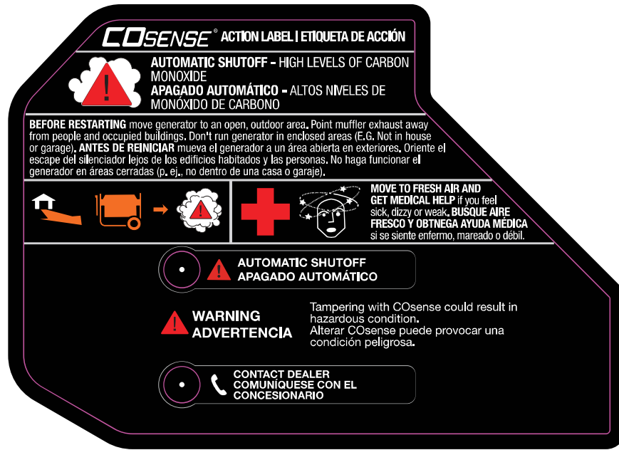
Figure 2-8. Instruction Action Label
